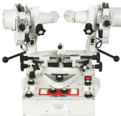
SYNOPTOPHORE
